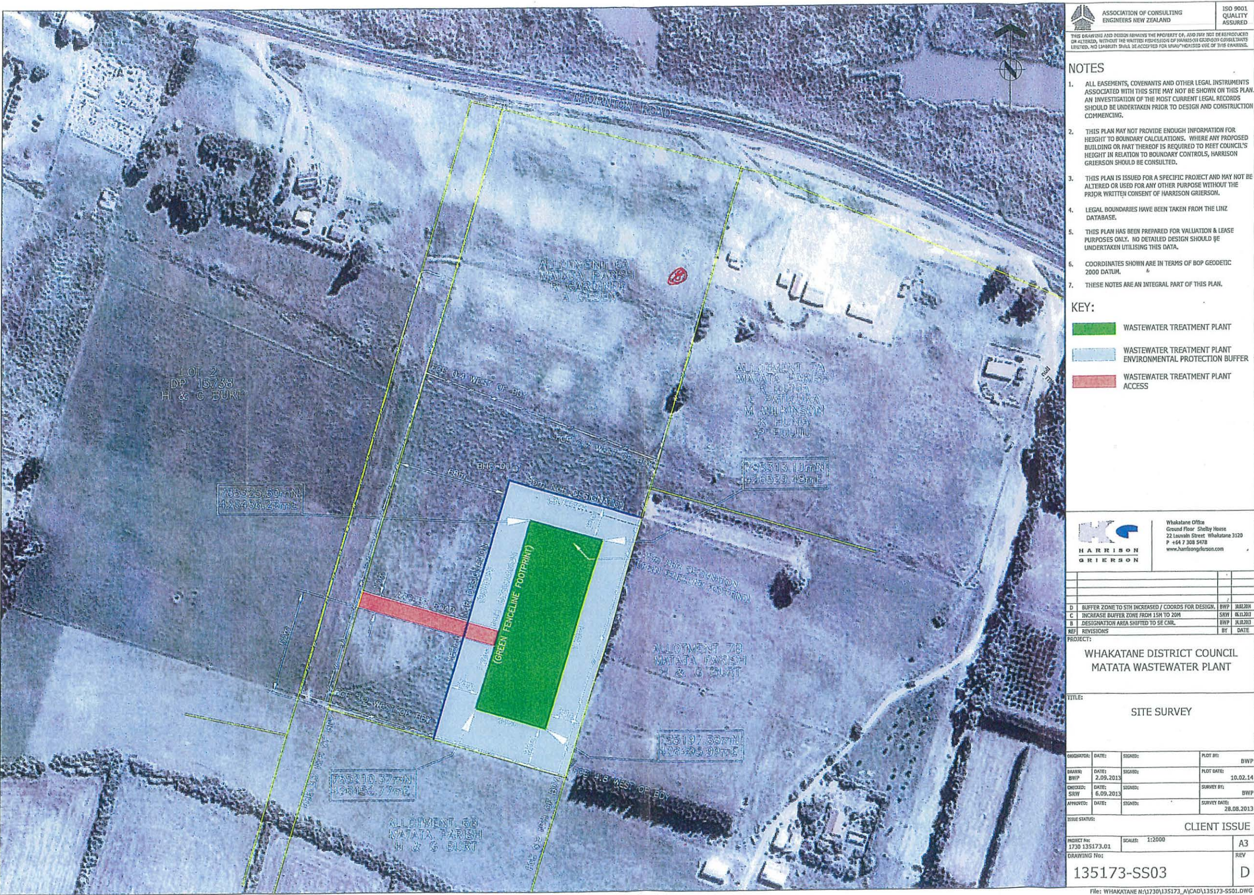
Figure 3: Layout of the Proposed Designation for the Wastewater Treatment Plant Site and Access Road
